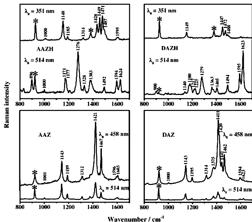
Figure 3. Raman spectra of neutral and cationic species of 4-amino- (AAZ/AAZH) and 4-(dimethylamino)azobenzene (DAZ/DAZH) in acetonitrile solutions at different excitation energies. Internal standard is at 920\text{ cm}^{-1} ( \text{CH}_3\text{CN} ).
